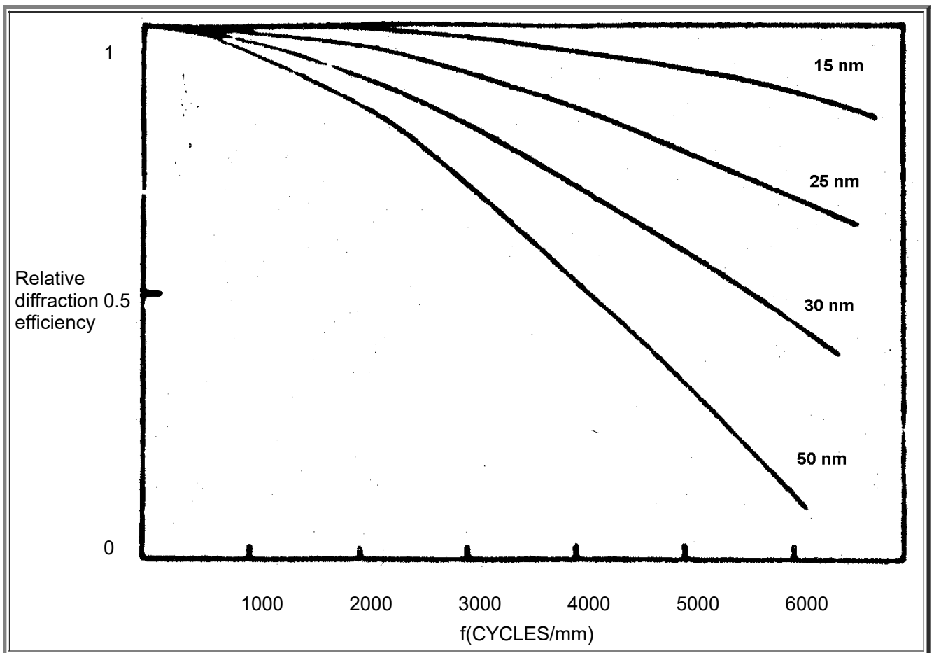
Figure 2: Calculated diffraction efficiency versus spatial frequency for different grain sizes [5].
