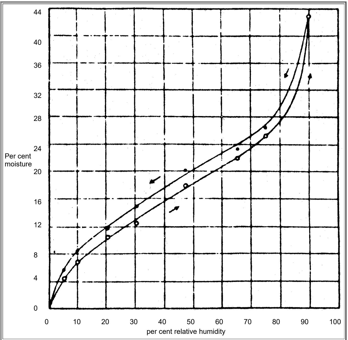
Figure 1: Relation between the moisture absorbed by dried gelatine and the relative humidity [7].
